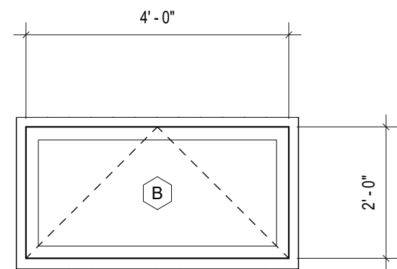
2 WINDOW TYPE B 1/2" = 1'-0"
